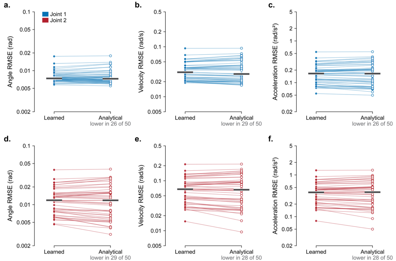
Supplementary Fig. 3 | Learned and analytical acceleration energies give median closed-loop simulation errors within 8% of each other.
